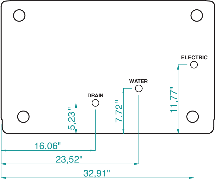
FRONT (BOTTOM VIEW)
